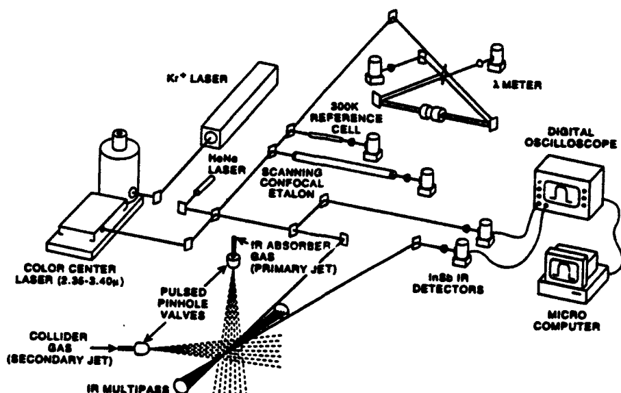
Fig. 1. Schematic of the current crossed jet apparatus for state-resolved energy transfer
